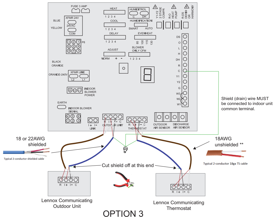
Figure 4. Lennox Communicating System Wiring Connections using Unshielded (Option 2) or Shielded Wiring (Option 3) Cabling
