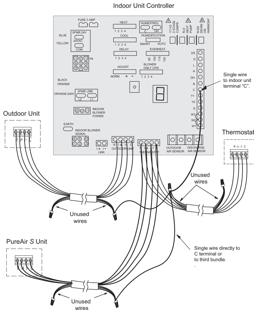
Figure 14. Unshielded Thermostat Cable (Multiple Conductors) used for Wiring Communicating Indoor Unit to PureAir S
