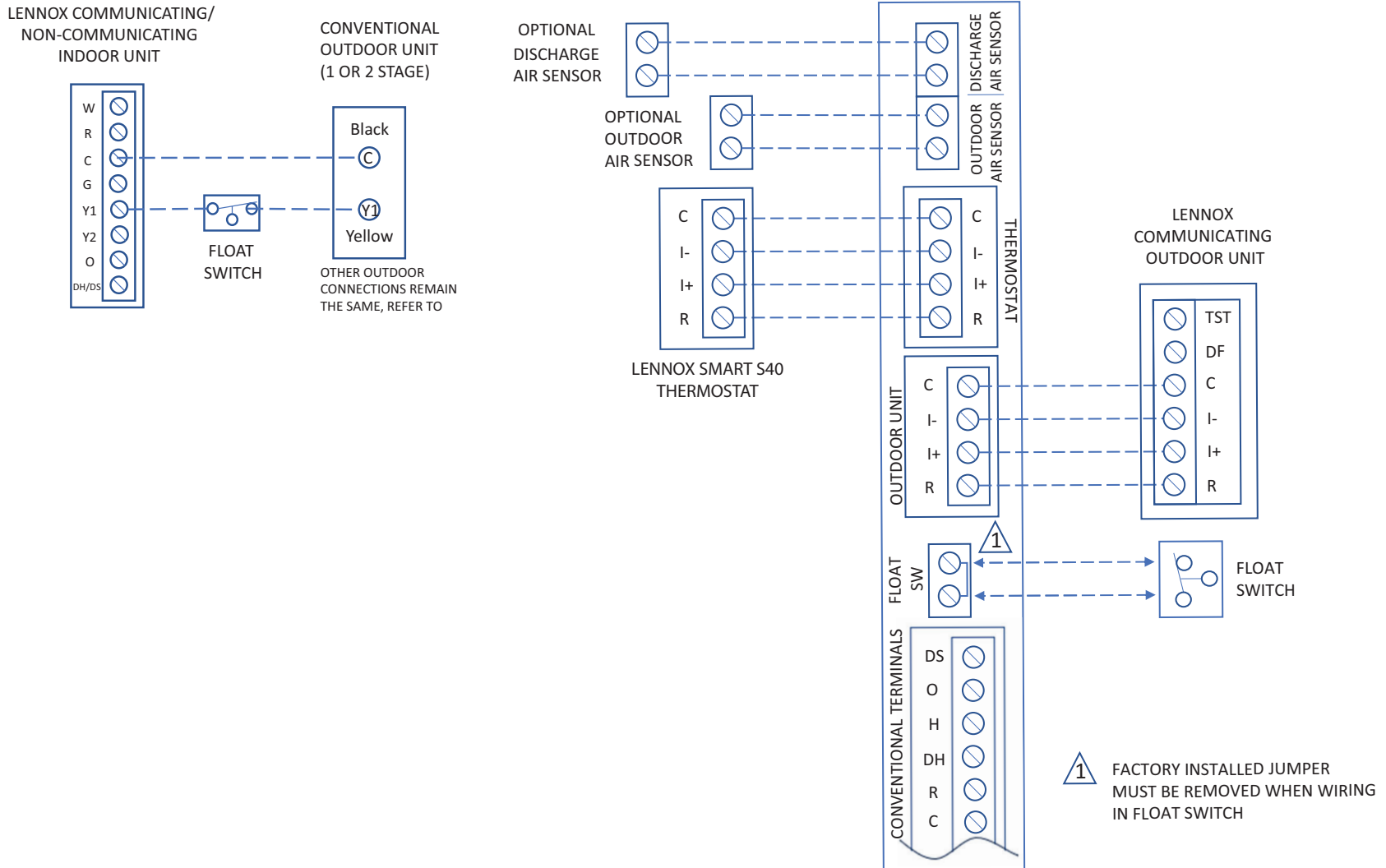
Figure 12. Lennox Smart S40, Lennox Communicating Indoor Controls and Float Switch
