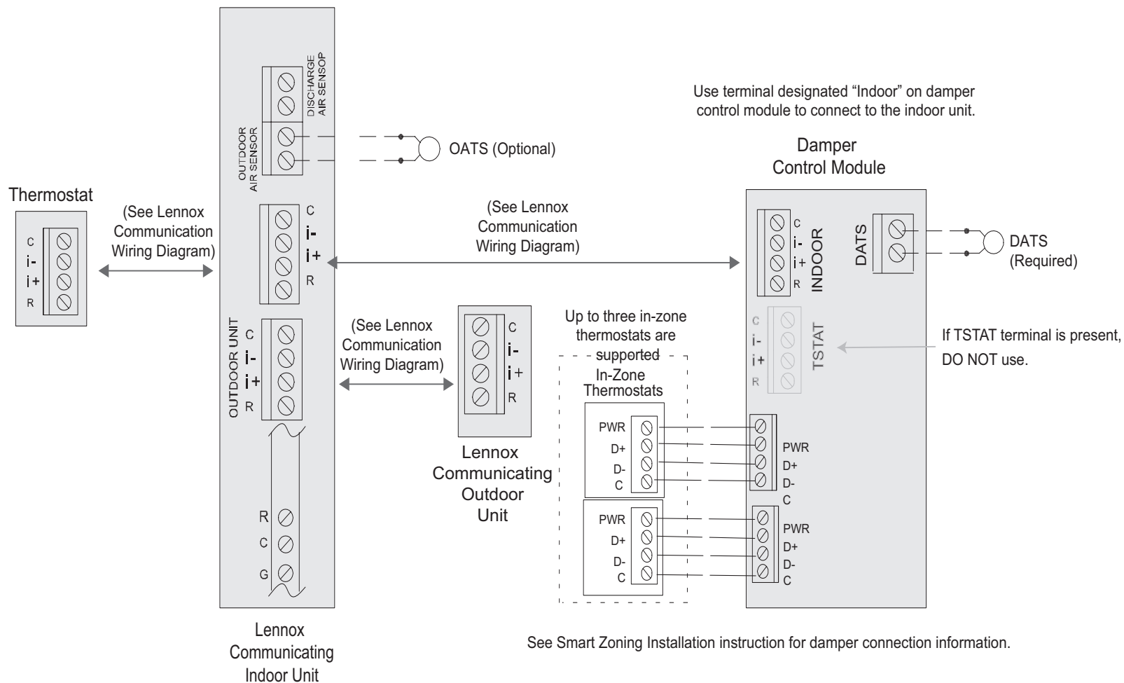
Figure 8. Lennox Smart S40, Lennox Communicating Indoor and Outdoor Units, Smart Zoning System (Damper Control Module) and Zone Sensors
