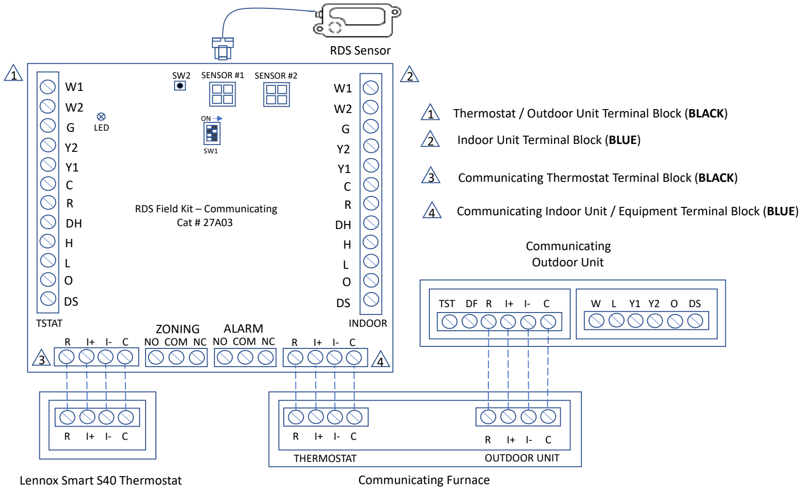
Figure 13. Lennox Smart S40, Lennox Communicating Non-Integral Gas Furnace Units with Low GWP Outdoor Unit and RDS Control
