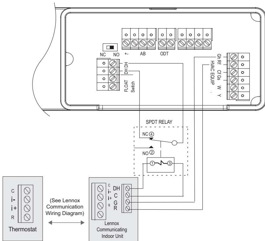
Figure 7. Lennox Smart S40, Communicating Indoor Control (Conventional Connections), Relay and HCWHD4 Series Dehumidifiers
