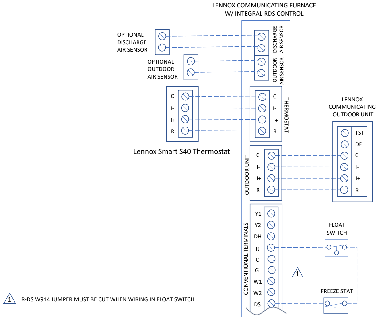
Figure 11. Lennox Smart S40 and HEPA Bypass Filter Interlock Kit and Humidifier
