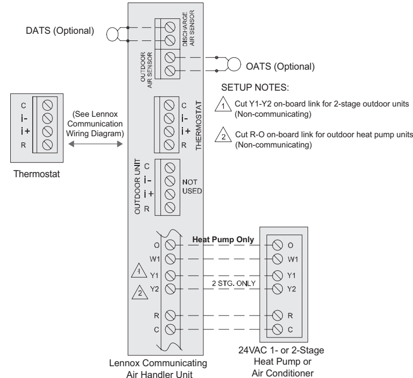
Figure 6. Lennox Smart S40, Lennox Communicating Air Handler with 24VAC (1- or 2-Stage) Heat Pump or Air Conditioner
