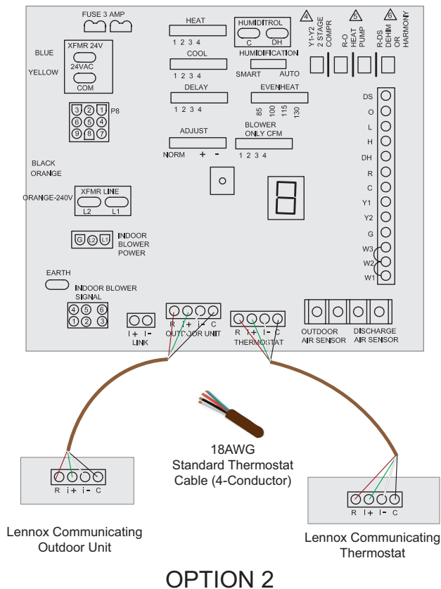
Figure 4. Lennox Communicating System Wiring Connections using Unshielded (Option 2) or Shielded Wiring (Option 3) Cabling
