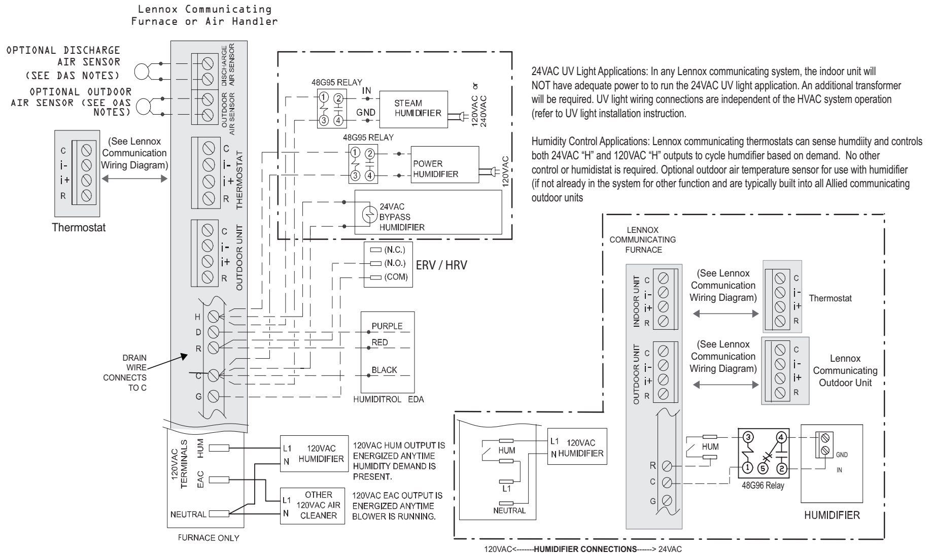
Figure 9. Lennox Smart S40 with Humidifier Accessory
